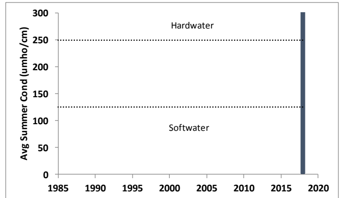
Specific Conductance
