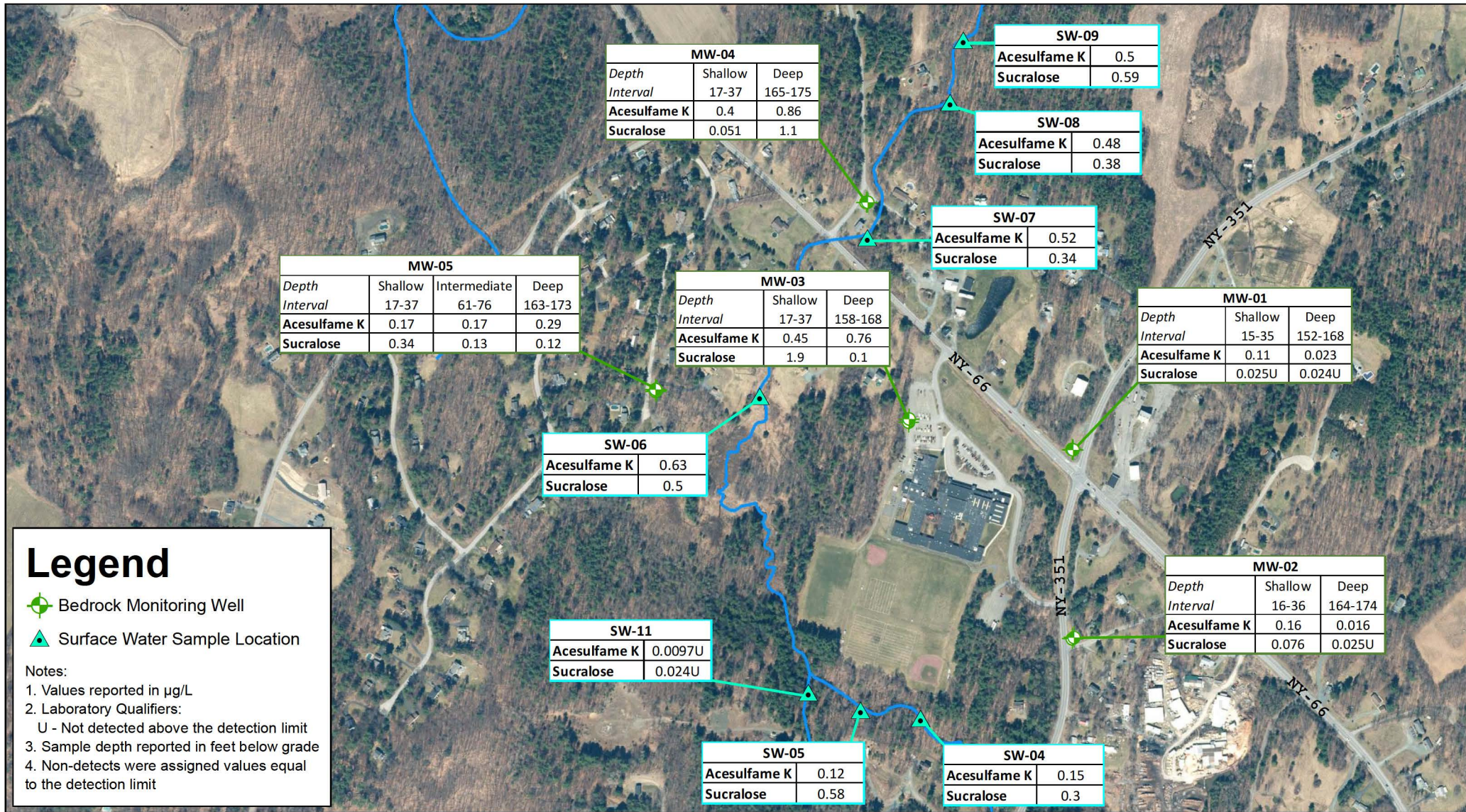
Poestenkill Assessment Area Surface Water and Bedrock Well Artificial Sweetener Results
