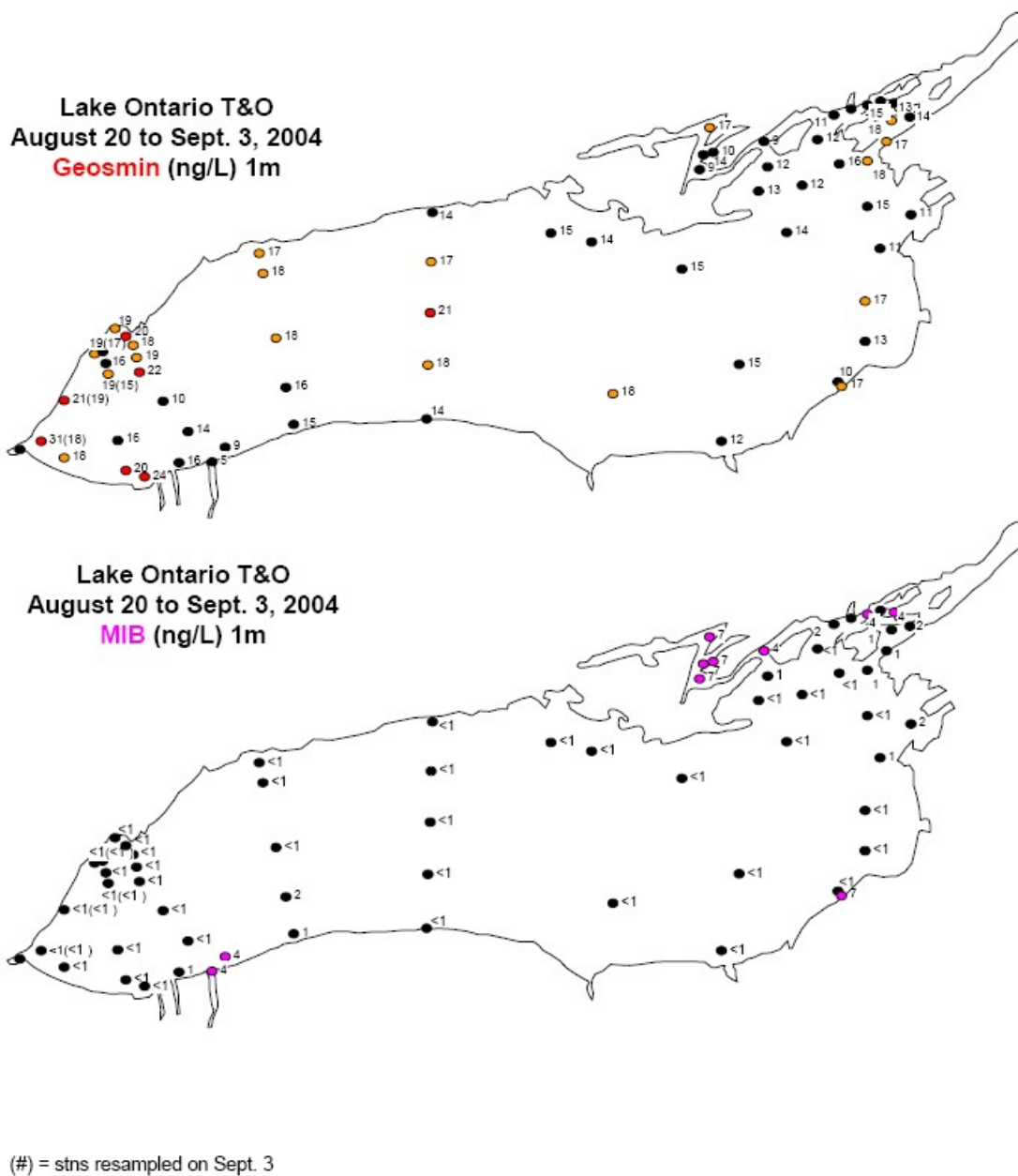
Fig. 13. Geosmin (above) and MIB (below) in the surface waters, Lake Ontario 2004. Higher values indicated in colour (red: geosmin > 20 ng/L; purple: MIB > 4 ng/L). Levels at stations sampled a second time during cruise indicated in brackets.
