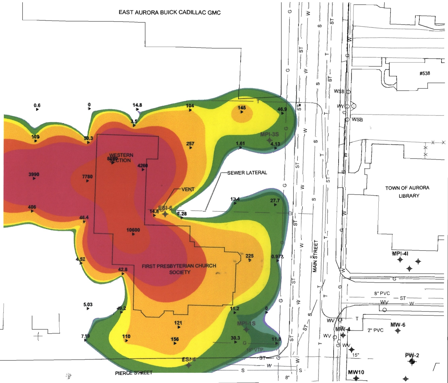
Total cVOC Concentrations in Soil Gas May 2004 East Aurora, New York
