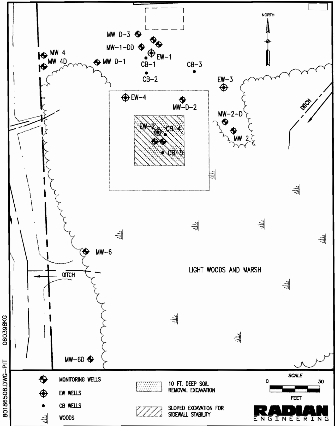
Figure 10: Alternative 3 - Excavation
