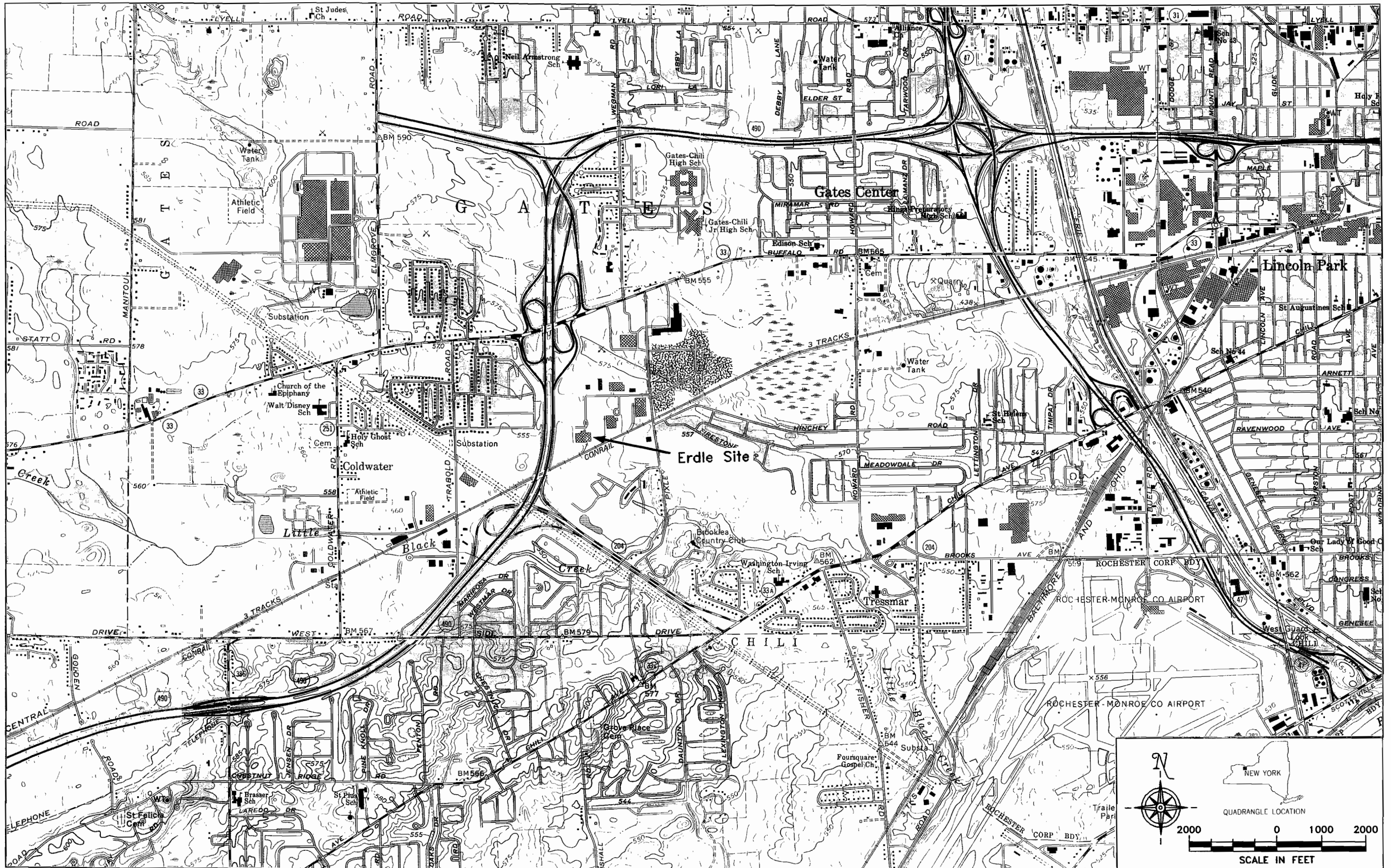
Figure 1-1. Site Topography
