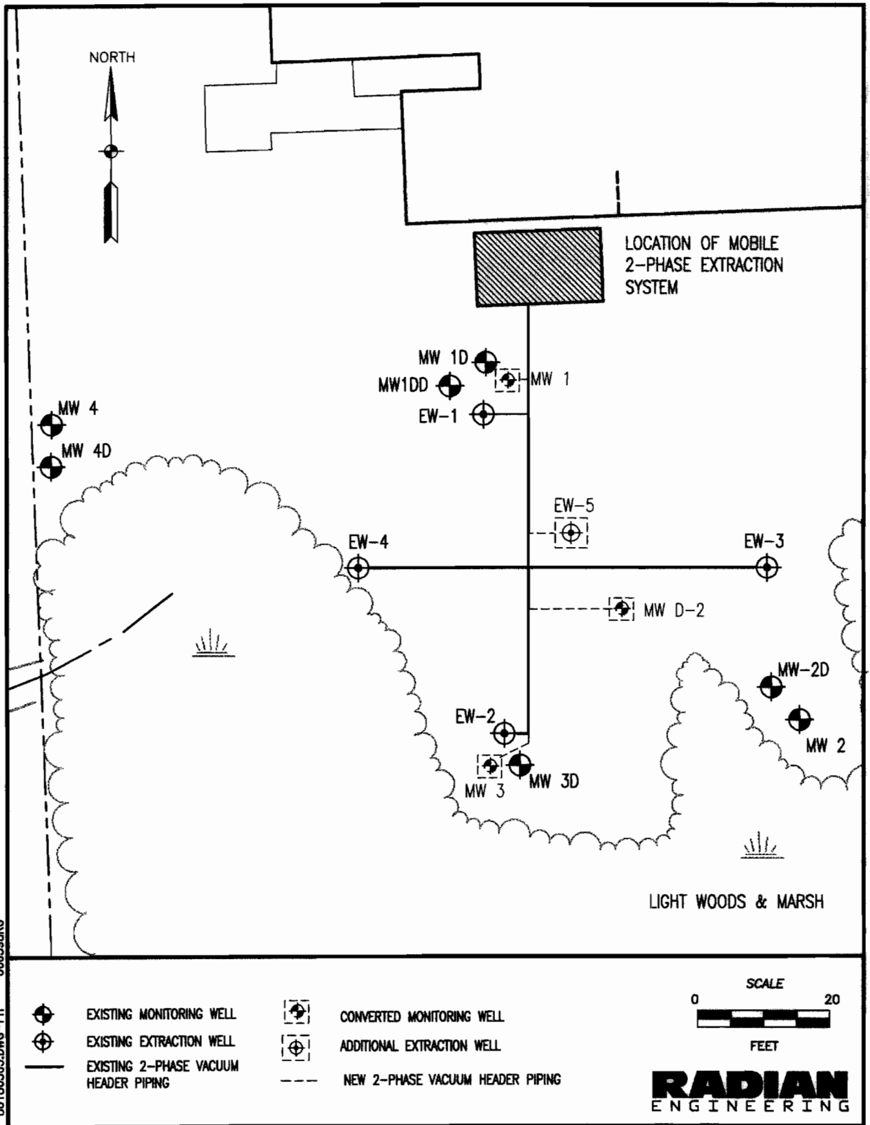
Figure 3: Expanded 2-PHASE Extraction System Layout
