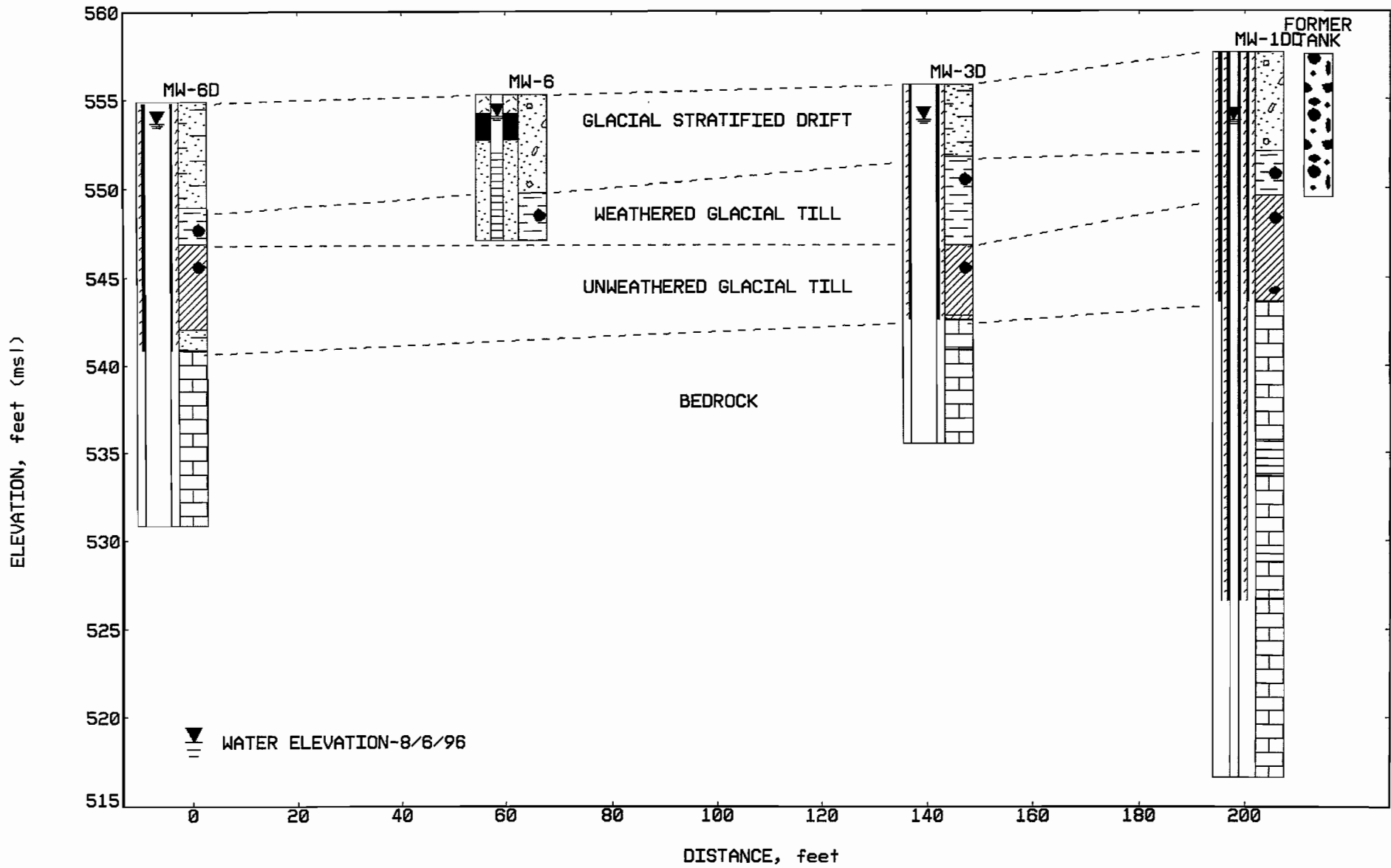
RADIAN Figure 3 PHASE II N-S CROSS SECTION 705-013 ERD2DTNS
