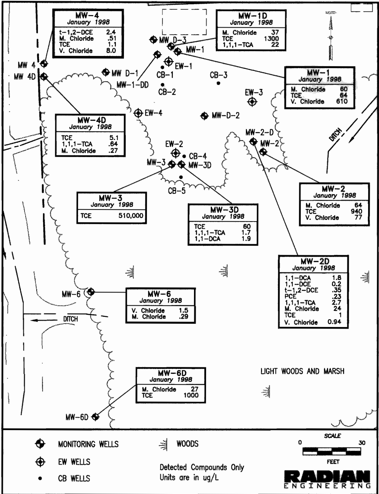
Figure 5 - Current Groundwater Concentrations
