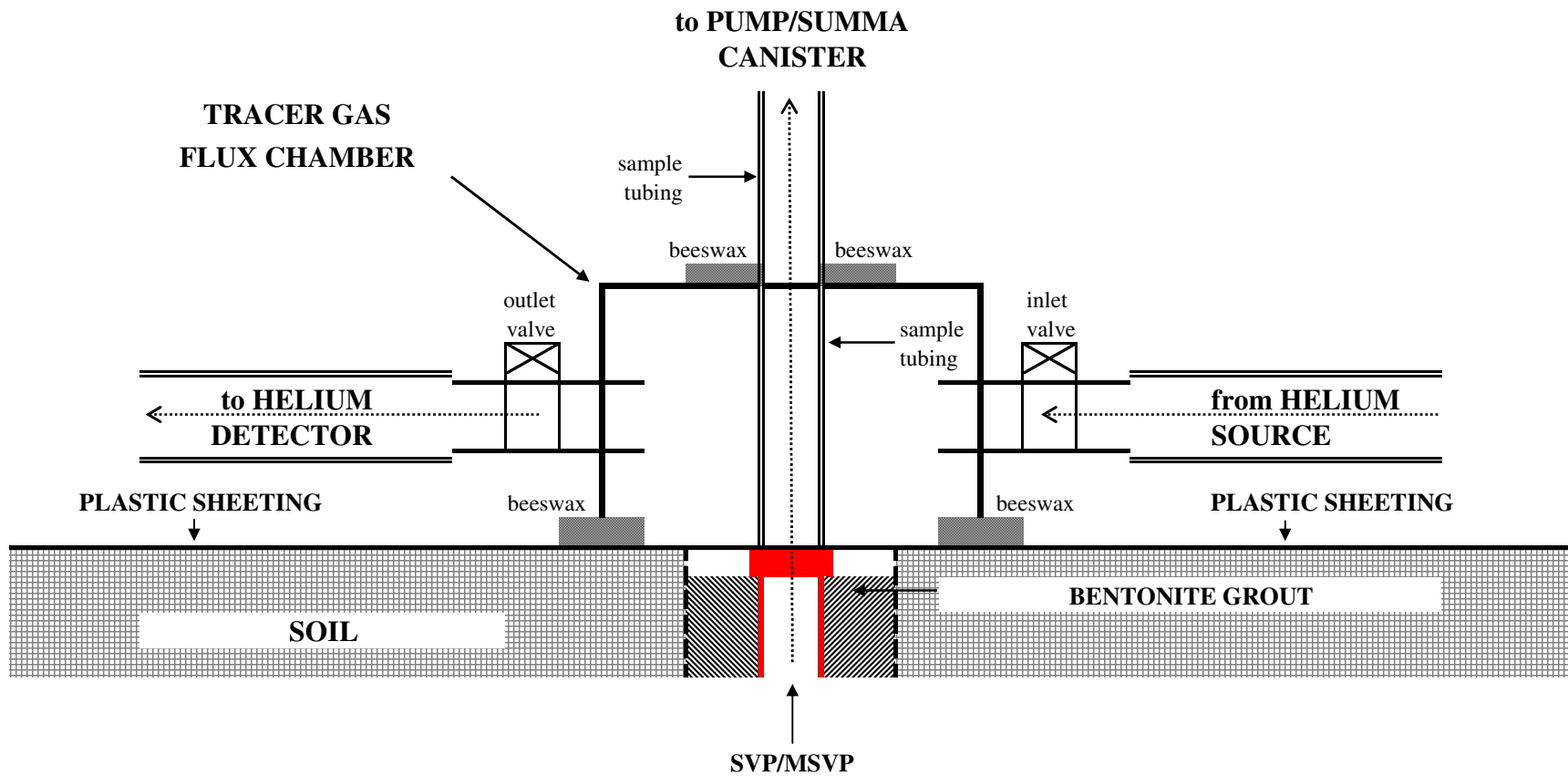
Figure 6-2 Tracer Gas Monitoring Chamber Schematic Former Norton/Nashua Tape Facility Watervliet, New York
