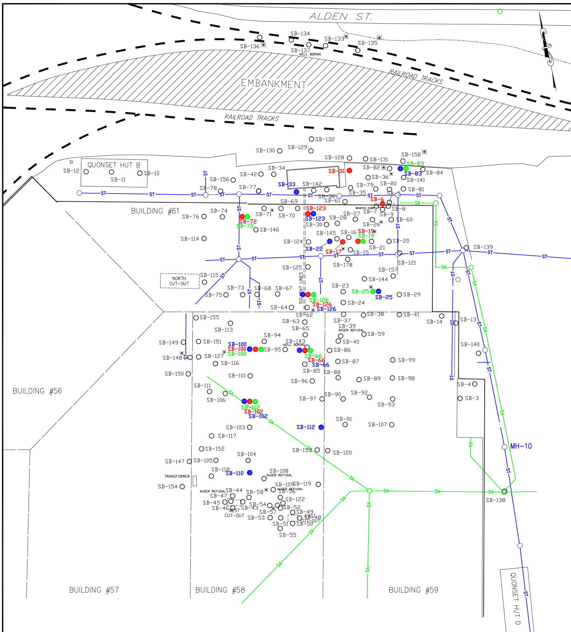
FORENSIC ENVIRONMENTAL SERVICES, INC. FIGURE 4-2 SOIL SAMPLING RESULTS (VOLATILES) FORMER NORTON/NASHUA TAPE PRODUCTS FACILITY WATERVLIET, NEW YORK SCALE IN FEET DRAWN BY: APPROVED BY:
