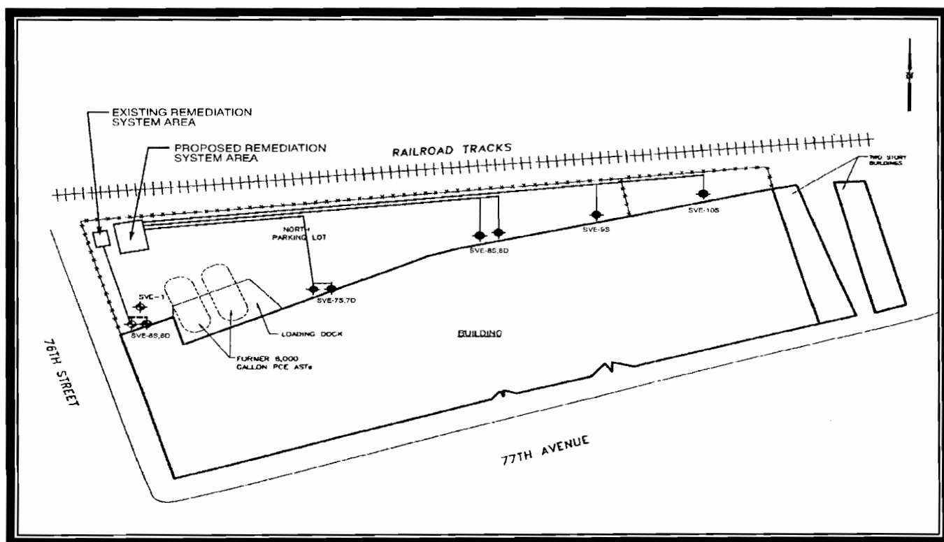
Figure 2 - Proposed SVE Well Locations and Treatment System Layout
