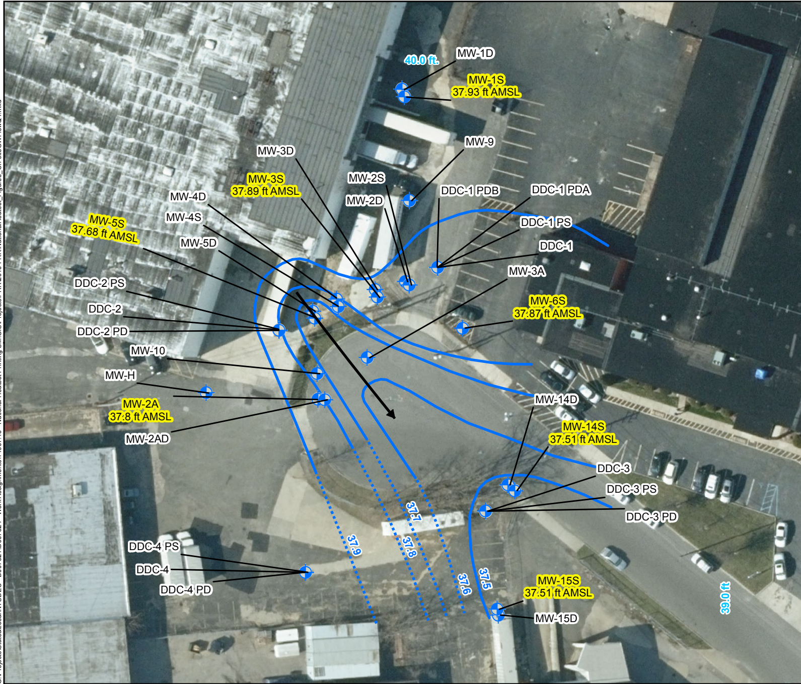
Figure 3 ON-SITE GROUNDWATER FLOW DIRECTION (October 2016) NATIONAL HEATSET SITE (152140) BABYLON, NEW YORK SUFFOLK COUNTY
