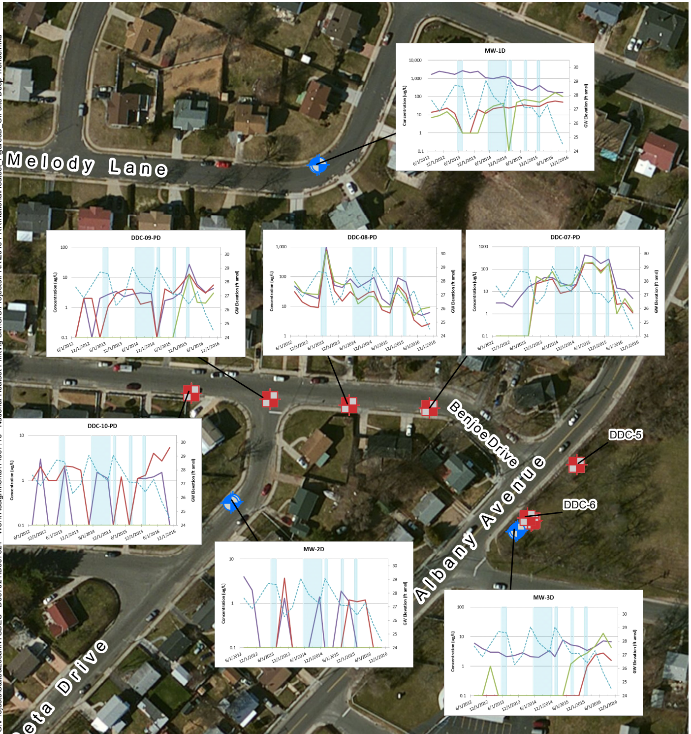
Figure 6D OFF-SITE DEEP WELLS CVOC TREND GRAPHS June 2012 - December 2016 NATIONAL HEATSET SITE (152140) BABYLON, NEW YORK SUFFOLK COUNTY
