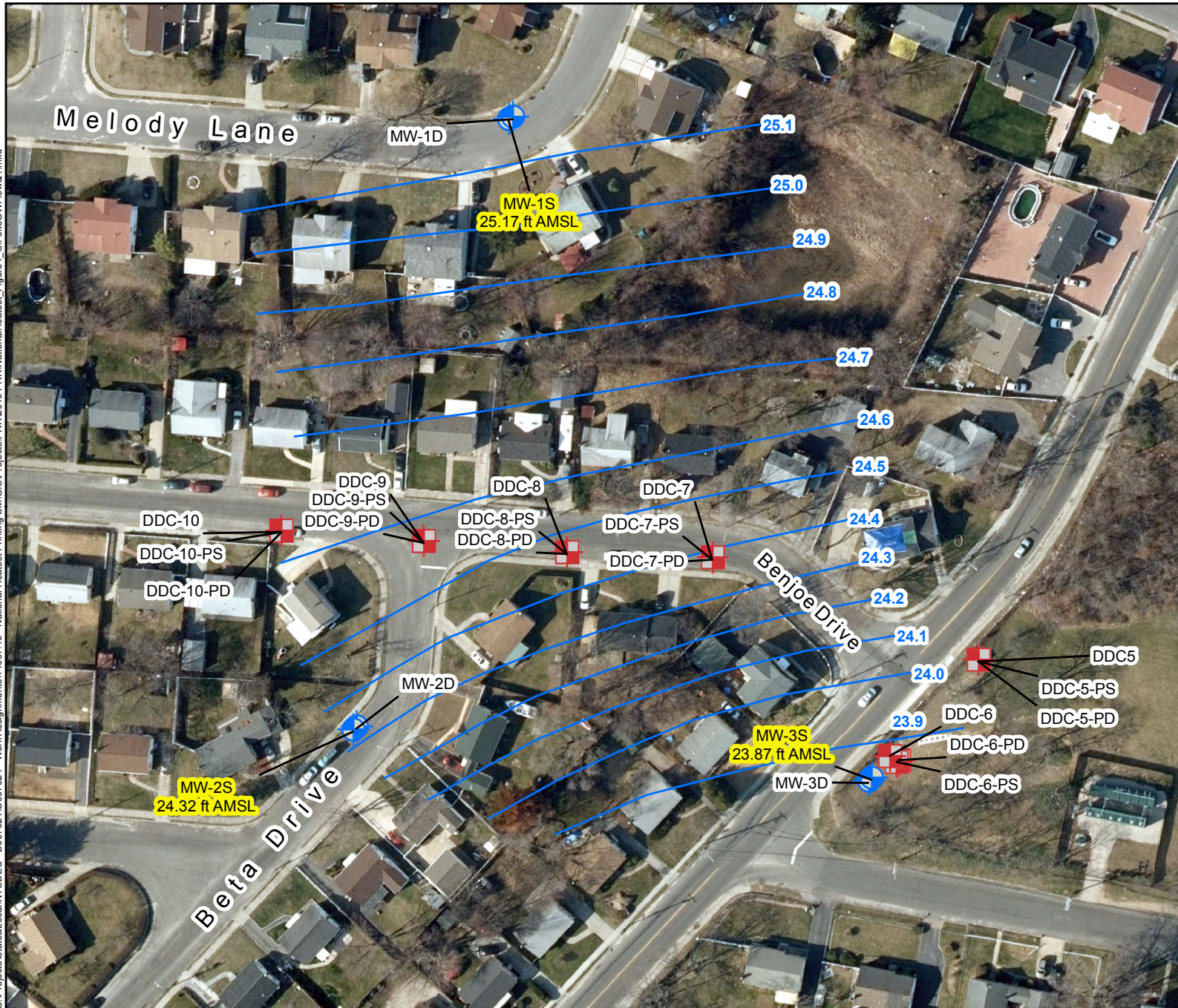
Figure 4 OFFSITE GROUNDWATER FLOW DIRECTION (October 2016) NATIONAL HEATSET SITE (152140) BABYLON, NEW YORK SUFFOLK COUNTY
