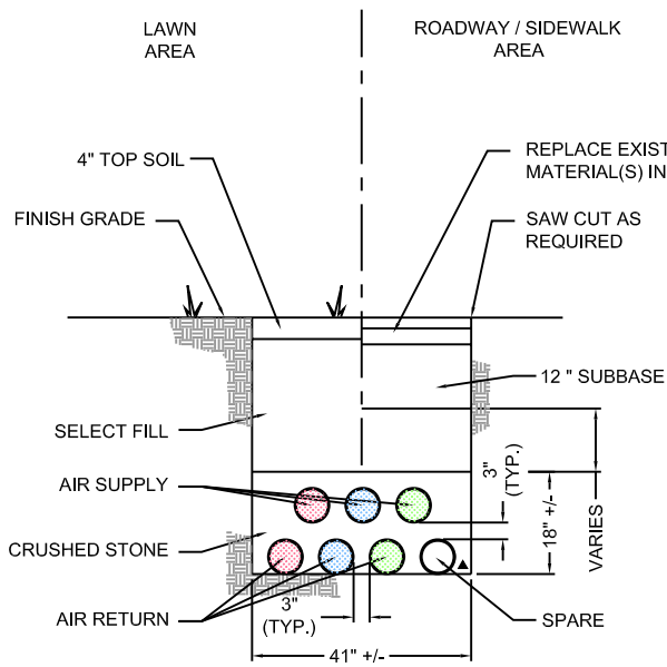
SECTION C-C TYPICAL 3 WELL SET TRENCH DETAIL
