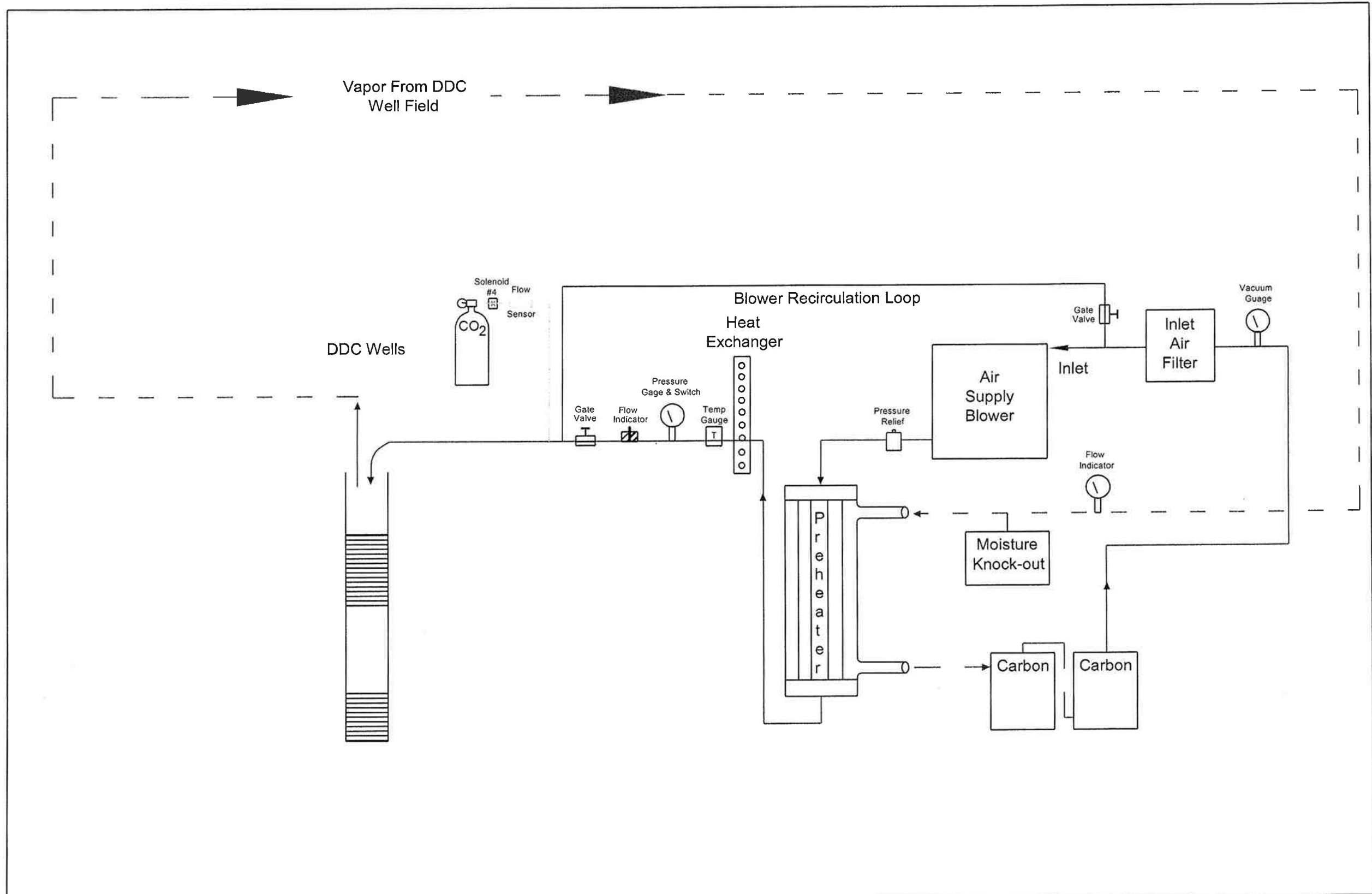
Figure 7 – Closed Loop Schematic
