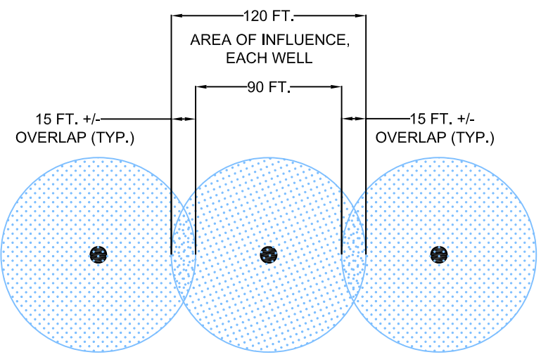
WELL LAYOUT DETAIL SCALE: NTS
