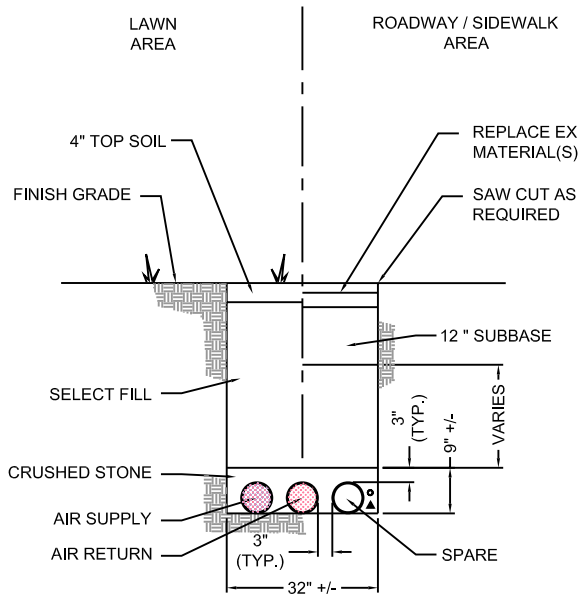
SECTION A-A TYPICAL 1 WELL SET TRENCH DETAIL
