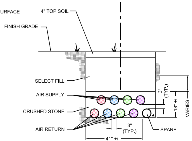
SECTION D-D TYPICAL 4 WELL SET TRENCH DETAIL
