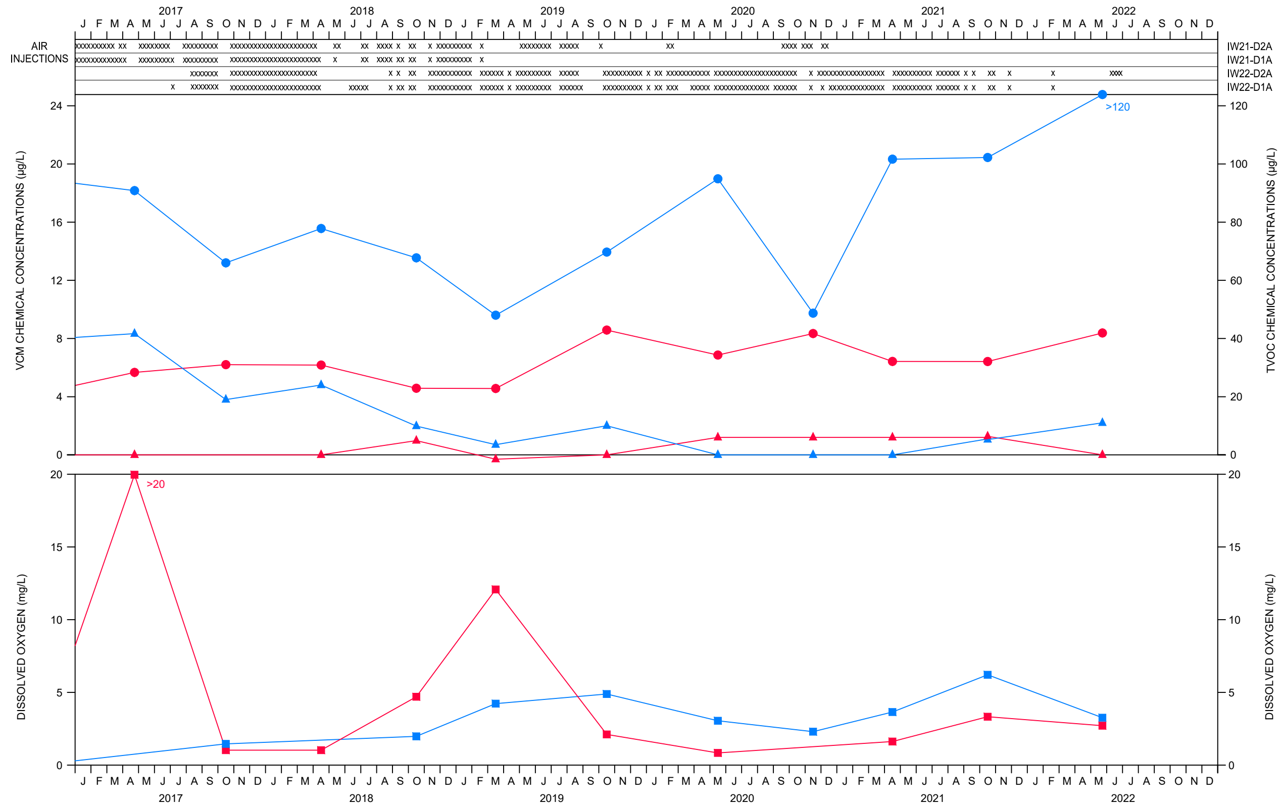
WELL NEST MW-89 CHEMICAL CONCENTRATION PLOTS MIDDLE INJECTION FENCELINE Hooker/Ruco Site, Hicksville, New York
