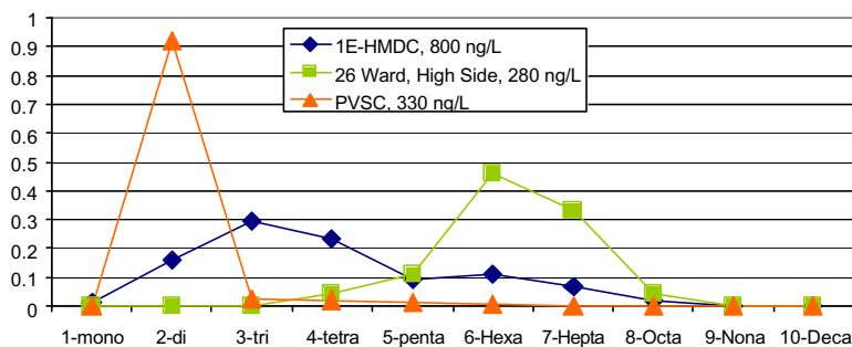
Figure 22. Relative abundances of PCB homologues from the three samples with the highest PCB concentrations.
