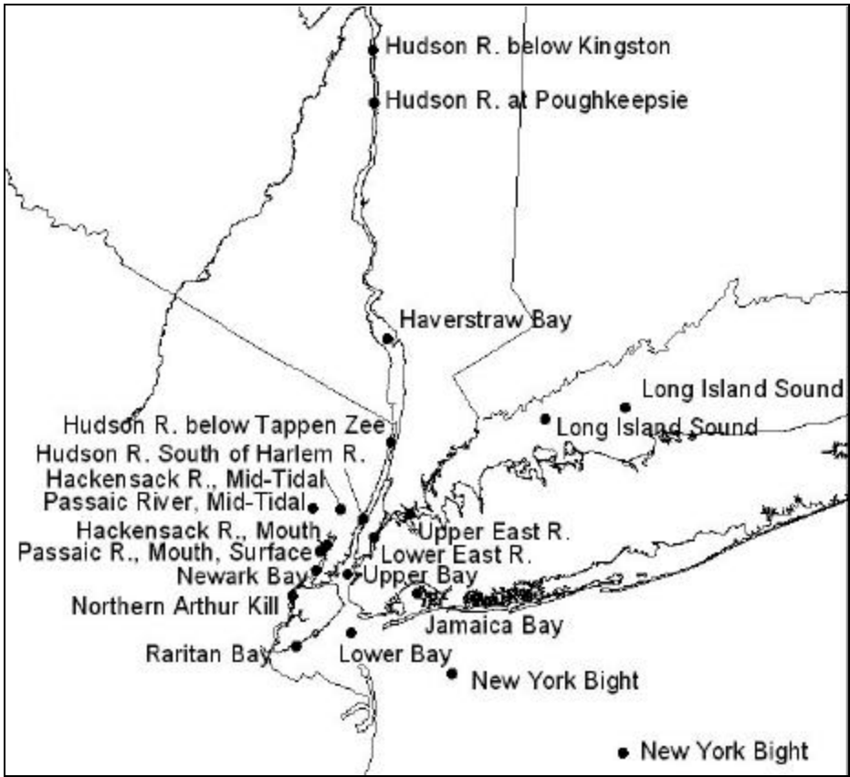
Figure 10. Centroids of ambient sampling stations.
