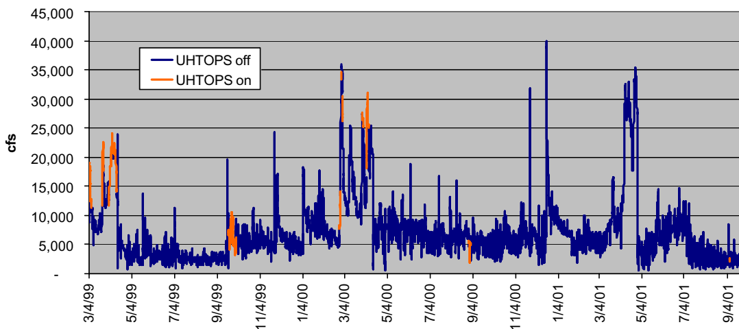
Figure 6. Over the period of study, TOPS was pumping while 7% of the Hudson's flow was passing.
