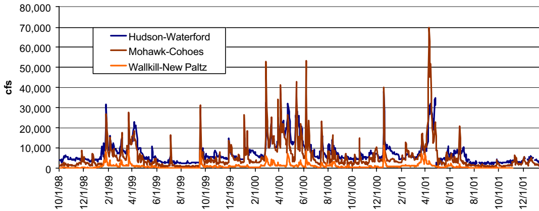
Figure 1. Comparison of discharges of the three largest freshwater sources to the Hudson Estuary over the life of CARP.
