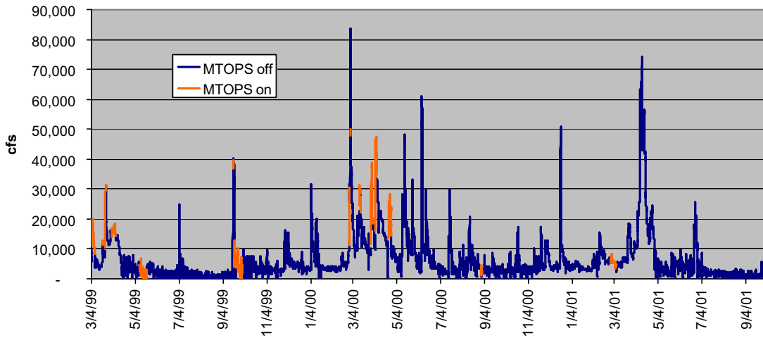
Figure 7. Over the study period, TOPS was pumping while 11% of the Mohawk's flow passed.
