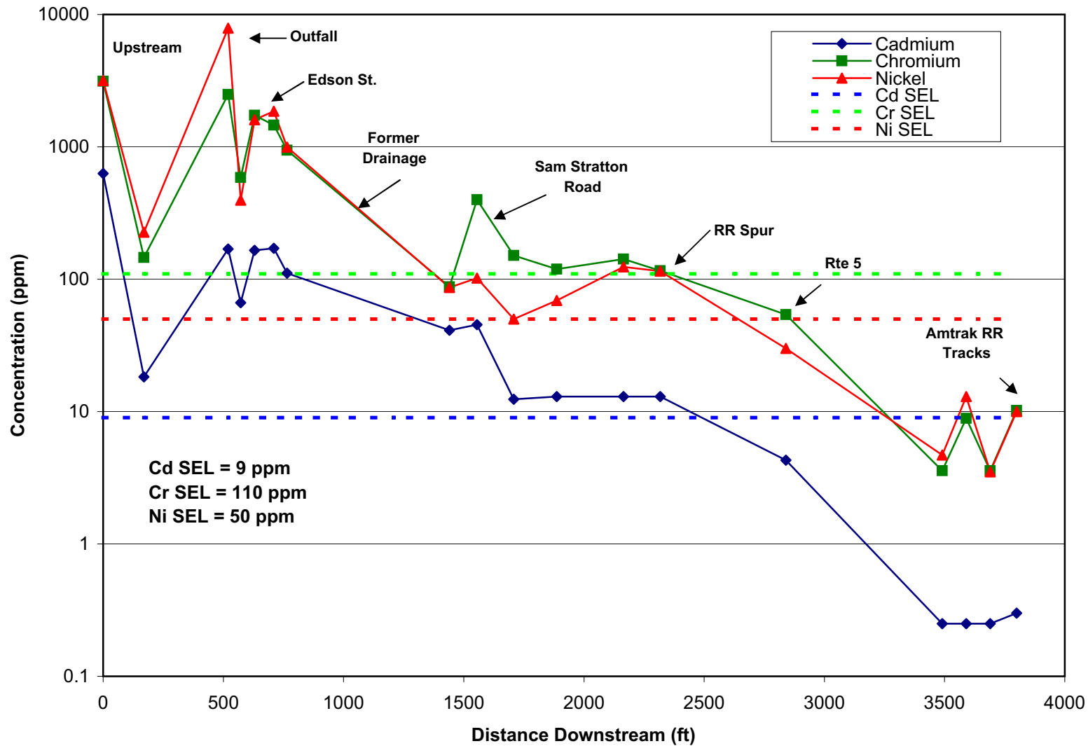
Figure 16 - Concentration of Cadmium, Chromium and Nickel in Sediment Samples Collected from the West Branch Drainage
