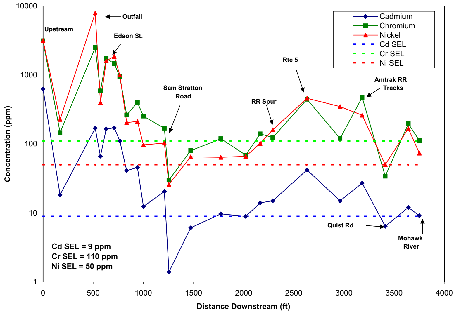
Figure 15 - Concentration of Cadmium, Chromium and Nickel in Sediment Samples Collected from the East Branch Drainage
