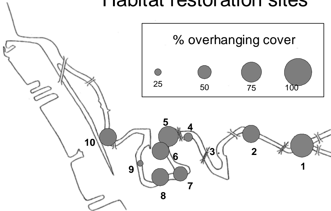
Figure 4.2 Percentage of shoreline with overhanging woody vegetation at potential habitat restoration sites.
