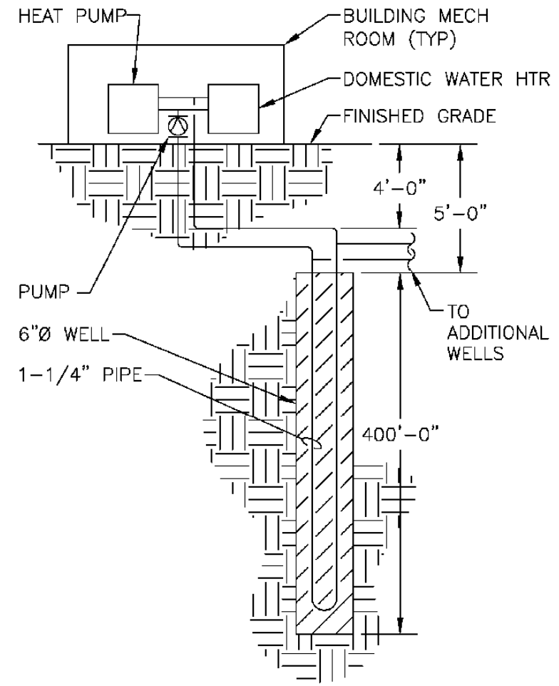
2 TYP WELL DETAIL SCALE: NTS
