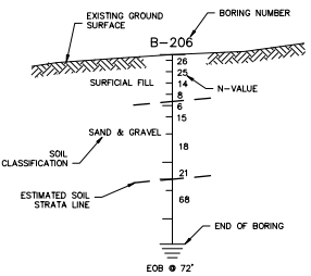
BORING LEGEND NOT TO SCALE
