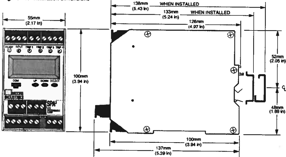
Figure 11. Installation Dimensions
