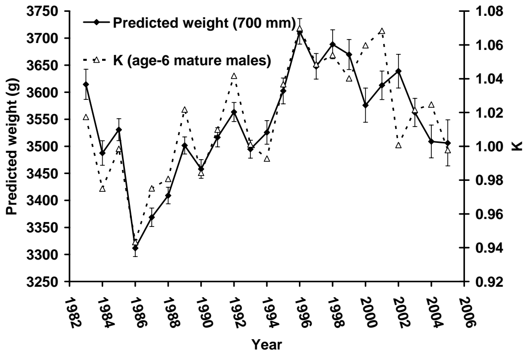
Figure 7. For Lake Ontario lake trout, condition ( K ) for age-6 mature males and predicted weight at 700-mm (27.6 in) TL from weight - length regressions calculated from all fish collected during each annual gill net survey, September 1983 – 2005. Error bars represent the regression confidence limits for each annual value.
