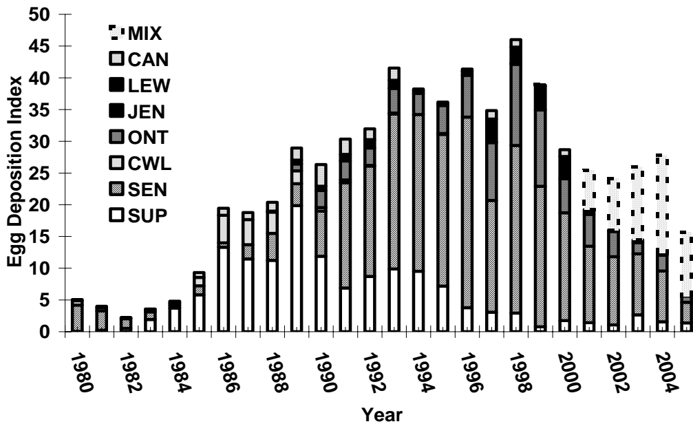
Figure 9. Egg deposition indices by strain (Strain descriptions for ONT, JEN, LEW, CWL, SEN, and SUP appear in Appendix 1) for lake trout in U.S. waters of Lake Ontario during 1980 - 2005. CAN represent a mix of the strains stocked by OMNR; and MIX represents values for untagged females stocked since 1997 for which strain could not be determined.
