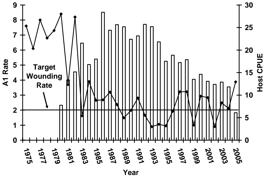
Figure 6. Wounding rates (A1 wounds per 100 lake trout, line) inflicted by sea lamprey on lake trout longer than 433 mm (17.1 in) TL collected from Lake Ontario in fall, 1975 – 2005. The CPUE of lake trout hosts (> 433 mm TL, bars) was calculated from index gillnet catches in September.
