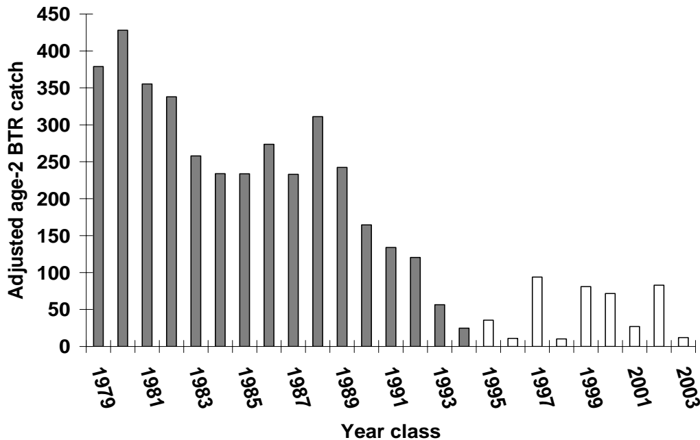
Figure 2. Survival indices for age-2 lake trout stocked as yearlings in U.S. waters of Lake Ontario in 1980 – 2004. Survival was indexed as the total catch per 500,000 fish stocked at age 2 from bottom trawls (BTR) fished in July-August (Note: White bars represent trawl data collected with the new trawl configuration which did not fish as hard on the lake bottom as the old trawl).
