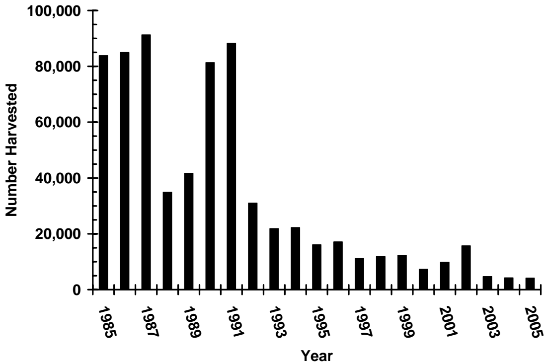
Figure 5. Estimated numbers of lake trout harvested by boat anglers from U.S. waters of Lake Ontario, 1985 – 2005 (Eckert 2006a).
