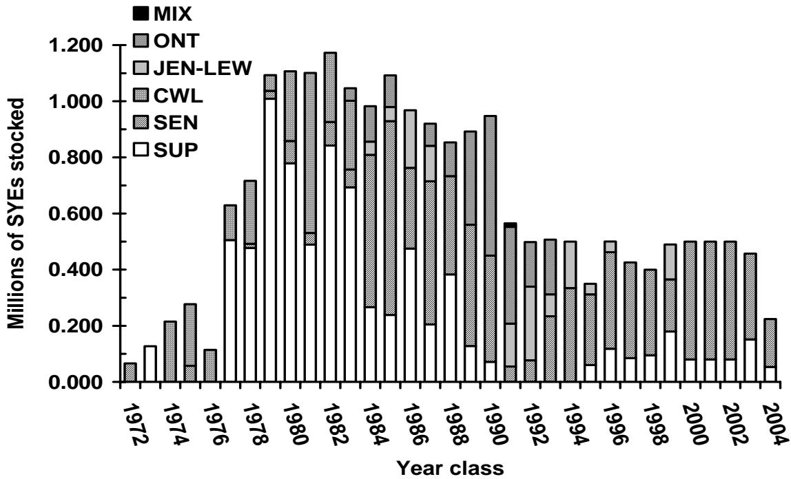
Figure 1. Total spring yearling equivalents (SYE) for lake trout strains (Strain descriptions for ONT, JEN-LEW, CWL, SEN, and SUP appear in Appendix 1) stocked in U.S. waters of Lake Ontario for the 1972 – 2004 year classes. MIX were unknowns. SYE = 1 spring yearling or 2.4 fall fingerlings (Elrod et al. 1988). Fall fingerlings were not stocked after 1991.
