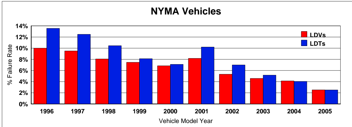
Graph 3: Calendar Year 2007 OBD II Inspection Failure Rates
